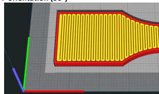
X-Y-orientation (90°)
