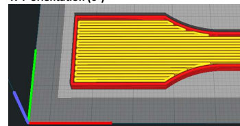
X-Y-orientation (0°)
