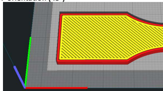
X-Y-orientation (45°)
