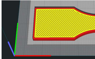
X-Y-orientation (45°)
